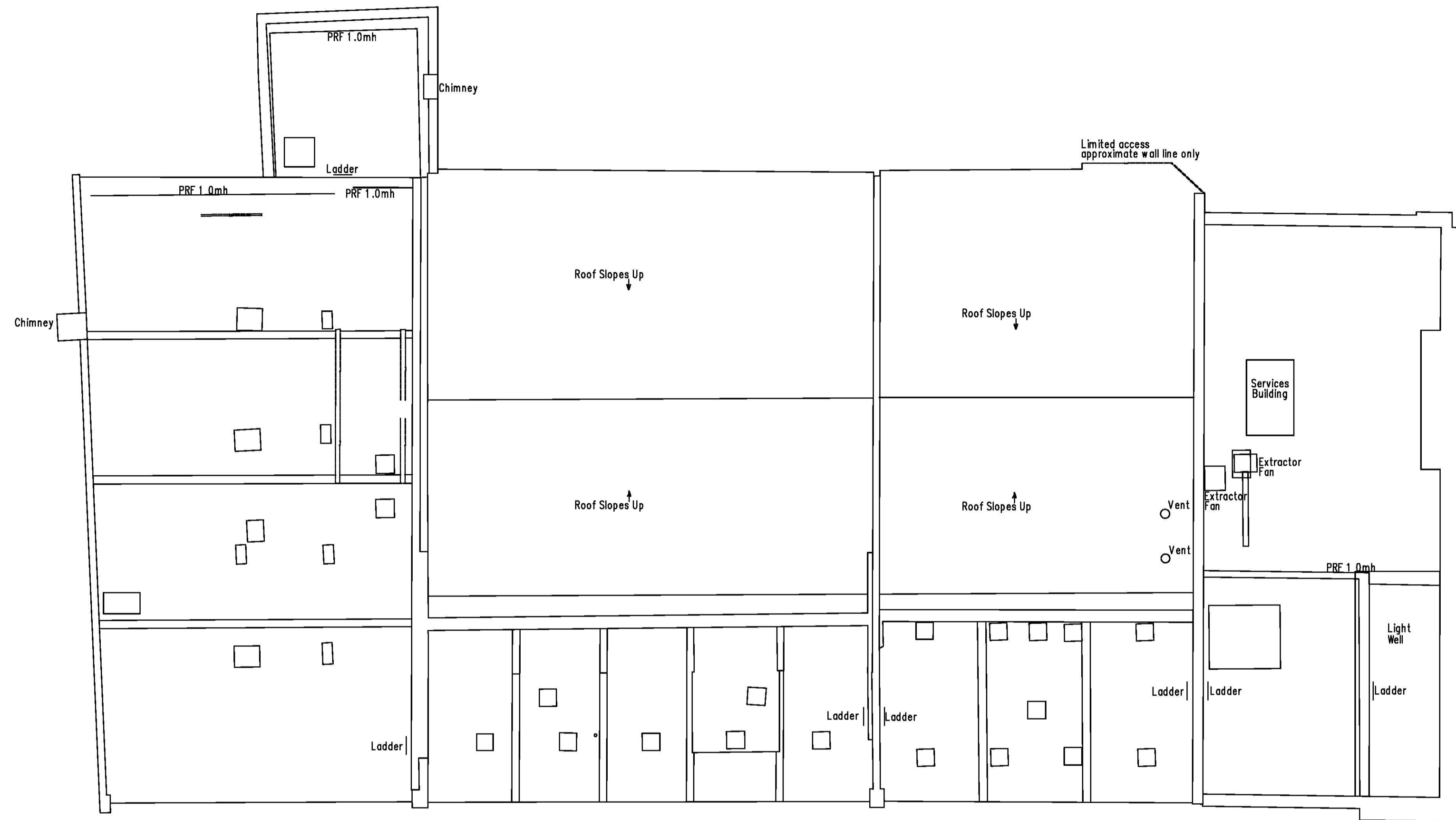
Existing Roof Plan Scale 1:100 @ A1
